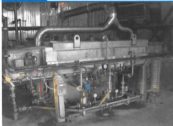
Filter press complete with vapor collection system.
